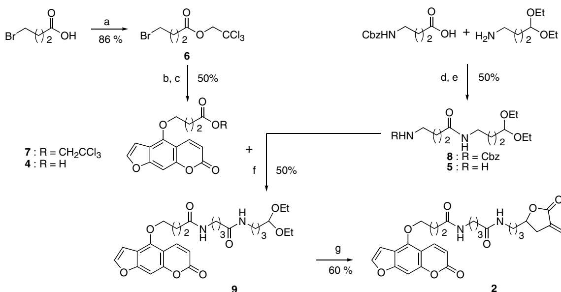
Scheme 1. Synthesis of 2 . Reagents and conditions: (a) 1.5 equiv \text{CCl}_3\text{CH}_2\text{OH} , 0.75 equiv p -TsOH, toluene, reflux, 58 h; (b) 0.9 equiv bergaptol, 1.3 equiv \text{K}_2\text{CO}_3 , acetone, reflux, 18 h; (c) 19 equiv Zn, AcOH, \text{CH}_2\text{Cl}_2 , rt, 19 h; (d) 1 equiv DCC, 0.9 equiv DMAP, \text{CH}_2\text{Cl}_2 , rt, 18 h; (e) Pd/C, 3.5 equiv ammonium formate, MeOH, rt, 6 h; (f) 1.2 equiv EDCI, 1.1 equiv DMAP, \text{CH}_2\text{Cl}_2 , rt, 6 h; (g) 1.6 equiv \text{SnCl}_2 \cdot \text{H}_2\text{O} , 1.6 equiv \alpha -bromomethacrylic acid, THF, \text{H}^+ , reflux, 48 h.
